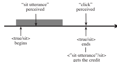
Figure 3: In this example, the \langle \text{"true"/sit} \rangle action tuple delegates credit to \langle \text{"sit-utterance"/sit} \rangle since the "sit-utterance" percept became active during the attention window (gray bar) associated with \langle \text{"true"/sit} \rangle and is a more novel and reliable predictor of reward than "true". By allowing the credit assignment phase to choose who gets credit we can dramatically simplify the learning and training process, as we will see in the section on action space discovery.
