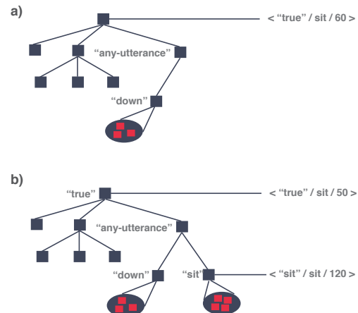
Figure 4: This figure illustrates the process of state-action space discovery. In (a) the trainer begins by rewarding the performance of <“true”/sit>, with the effect being that the reliability and value of <“true”/sit> increases. This in turn increases the frequency of sitting. Once the dog is sitting frequently, the trainer starts saying “sit” as the sit action is performed, while continuing to reward the sit. As the trainer continues this process, the system begins to build a classifier for the specific utterance that occurs during the attention window associated with rewarded sits, and eventually spawns a <“sit-utterance”/sit> percept-action pair (b). Over time the trainer will stop rewarding spontaneous sits or sits in response to other utterances (i.e., <“true”/sit> or <“any-utterance”/sit>). The effect is that the reliability (and value) of these action tuples will drop in comparison with that of <“sit-utterance”/sit> and these less specific and reliable action tuples are expressed less frequently.
