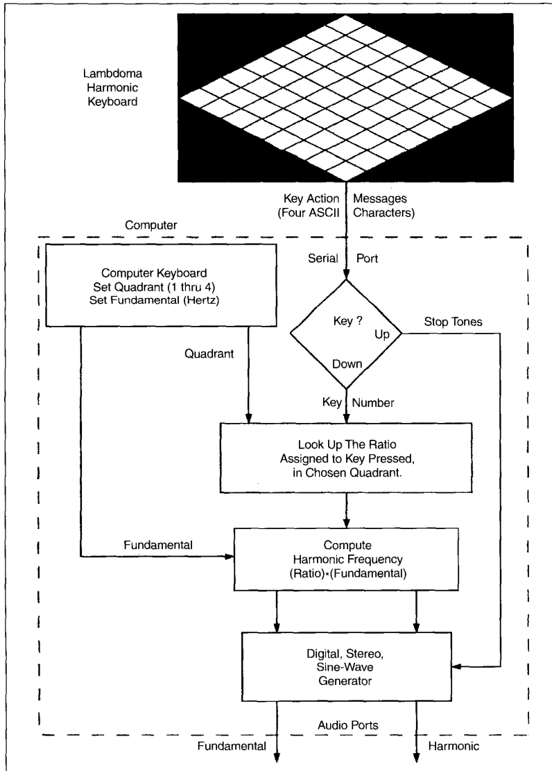
7. Flow diagram of the Lambdoma harmonic keyboard.
