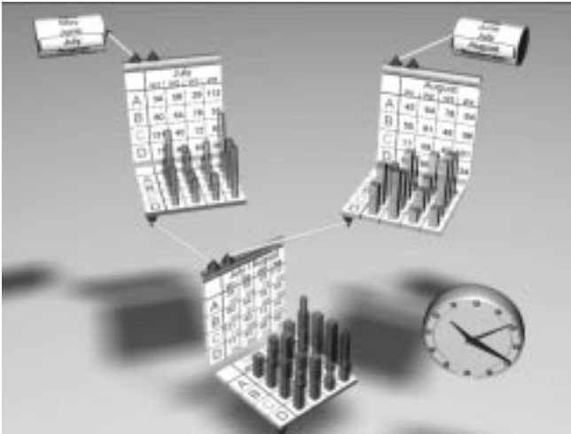
Fig. 3. The user-accessible software modules provide synapses (docks). Pipelines between the docks enable the transfer of information and allow the user to create complex applications (in this example a multidimensional spreadsheet) by visually connecting the docks of basic components.
