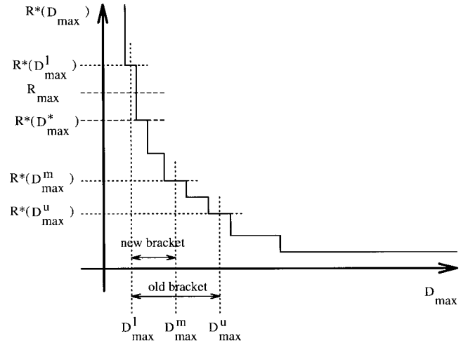
Fig. 1. The R^*(D_{\max}) function.
