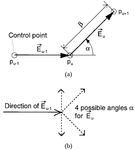
Fig. 16. Encoding of a spline control point.
