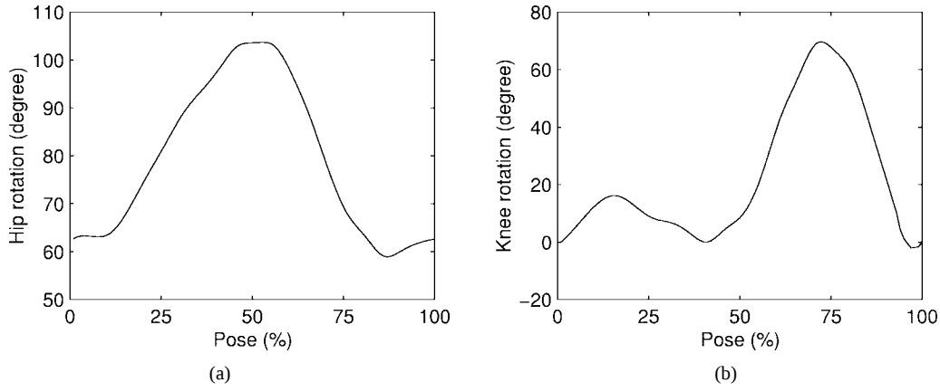
Fig. 3. Temporal walking curves: (a) hip angle \theta_{M3} ; (b) knee angle \theta_{M5} .
