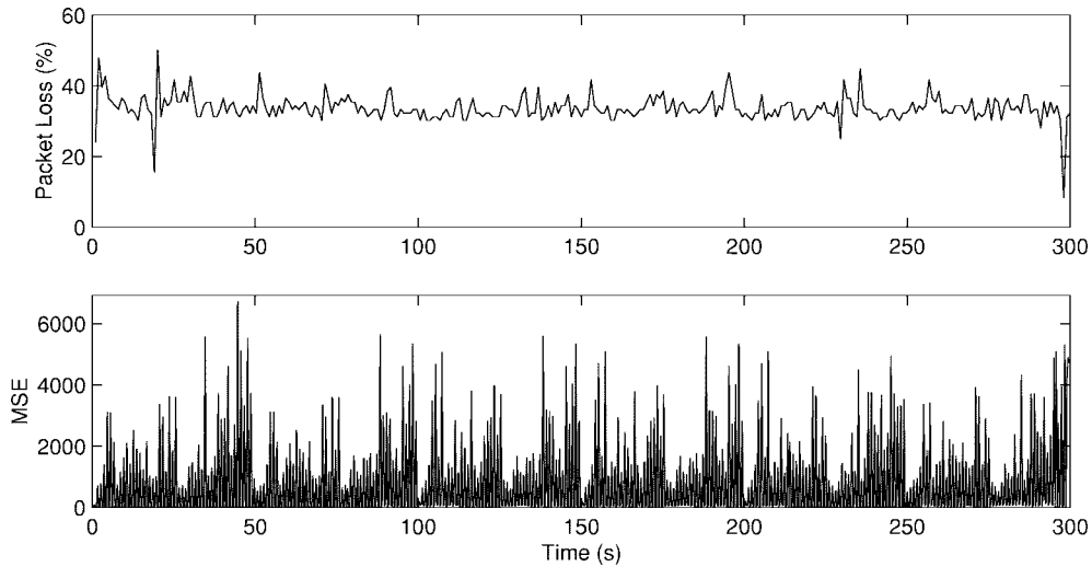
Fig. 11. Nonadaptive flow at 1 Mbps from Hong Kong to Berkeley using scheme (T) (2 pm, 9/8/98).
