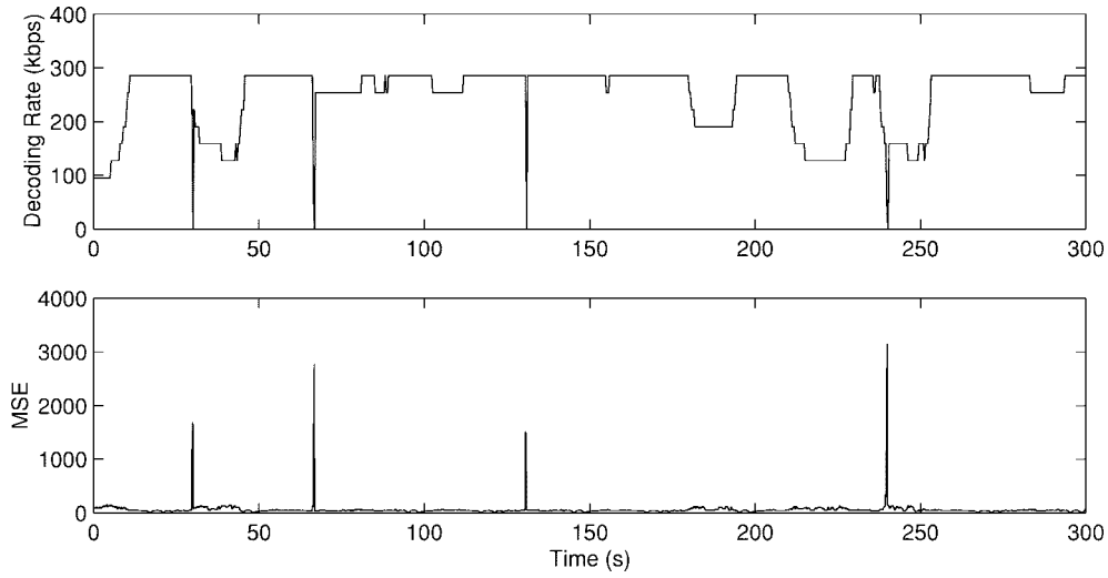
Fig. 12. Adaptive flow from Hong Kong to Berkeley using scheme (T) (3 pm, 9/8/98).
