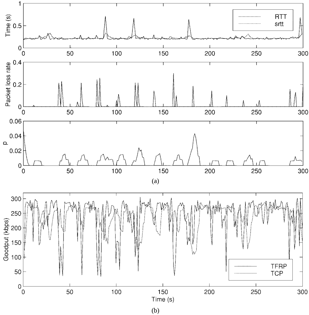
Fig. 13. Simultaneous transmission using TCP and TFRP between Hong Kong and Berkeley. First graph in (a) shows instantaneous RTT and the average RTT ( srtt ). The second graph in (a) shows packet loss rate observed at the receiver. The third graph in (a) shows p as estimated at the sender. (b) Bandwidth consumes by TCP and TFRP.
