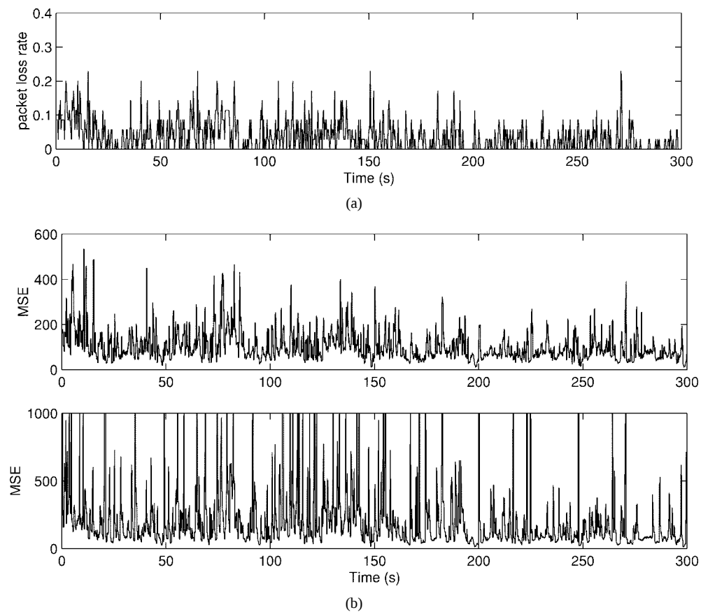
Fig. 16. Simultaneous video transmission from Hong Kong to Berkeley with rate-control (3 pm on 10/20/98). (a) Loss rate. (b) Corresponds to MSE for schemes (P) and (T), respectively.
