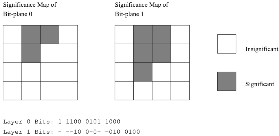
Fig. 3. Coding significance maps using hierarchical block coding. “-” indicates values that can be deduced.
