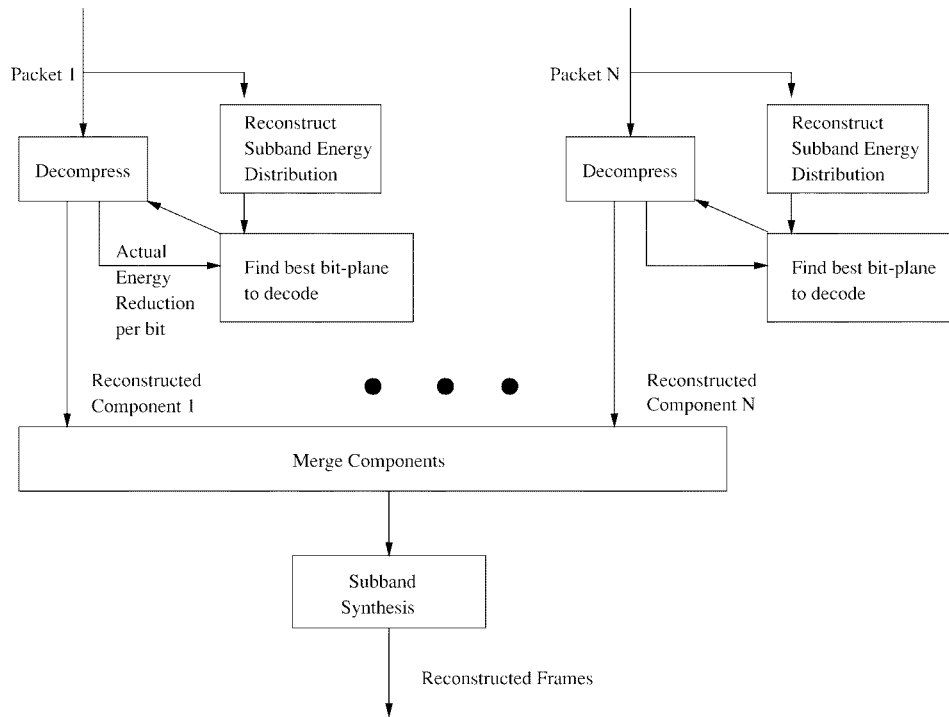
Fig. 6. Decoding procedures.
