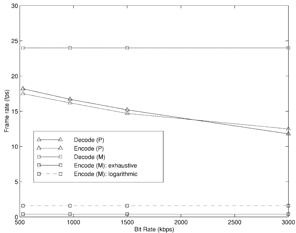
Fig. 8. Speed comparisons of the proposed scheme (P) and MPEG-1 (M) on an 170 MHz Ultra-sparc. “Exhaustive” and “logarithmic” refer to the different strategies in motion estimation of MPEG.
