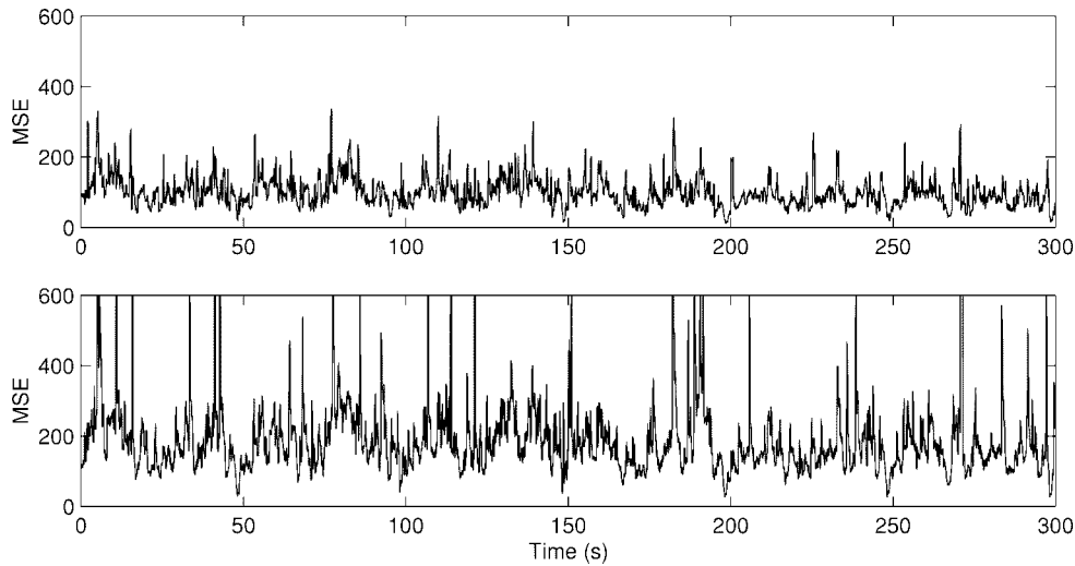
Fig. 18. Simultaneous video transmission from Hong Kong to Berkeley using TFRP and adaptive FEC. Top is scheme (P) and bottom is (T).
