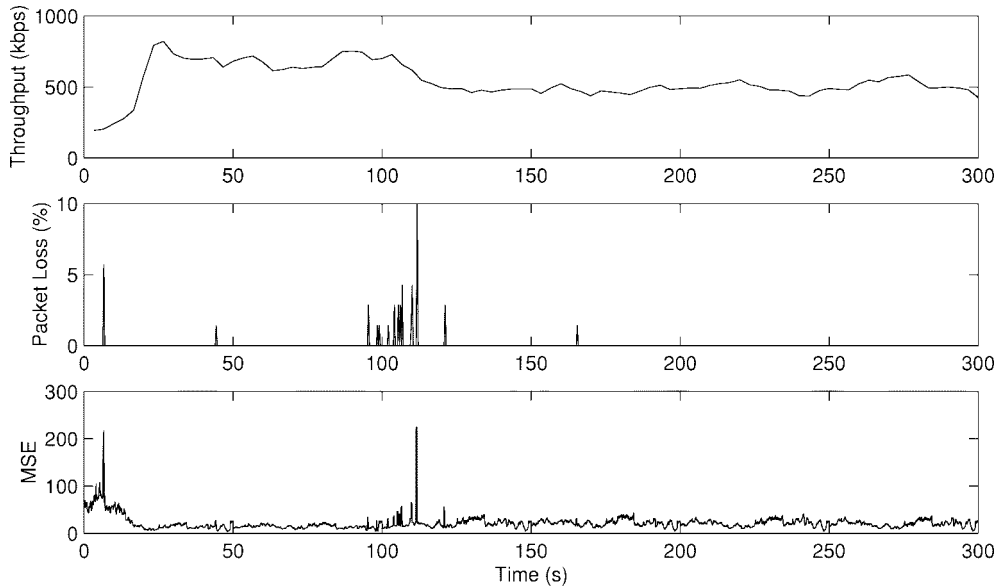
Fig. 15. Throughput (top), packet loss rate at receiver (middle) and video quality (bottom) for the proposed compression scheme (P) with TFRP from Toronto to Berkeley (6 pm, June 23, 1998).
