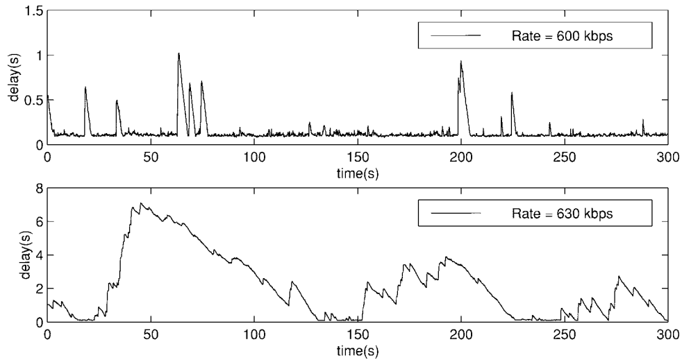
Fig. 10. Delay for video transport using TCP from Toronto to Berkeley (noon, May 11, 1998).
