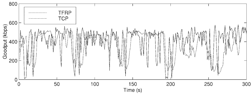
Fig. 14. Throughput of simultaneous transmission of TCP and TFRP from Toronto to Berkeley.
