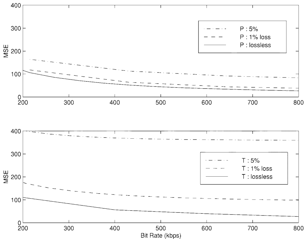
Fig. 17. Distortion-rate characteristics of schemes (P) and (T) at 0, 1, and 5% packet loss.
