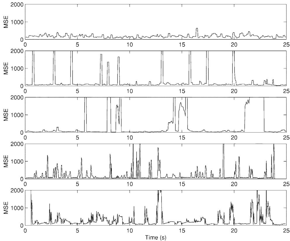
Fig. 7. Variability of quality at 5% simulated random packet loss. From top to bottom: (P), (S), (T), (M) with GOP 2, (M) with GOP 15.
