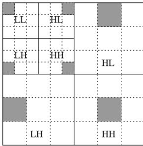
Fig. 2. Grouping coefficient blocks from different subbands to form a component.
