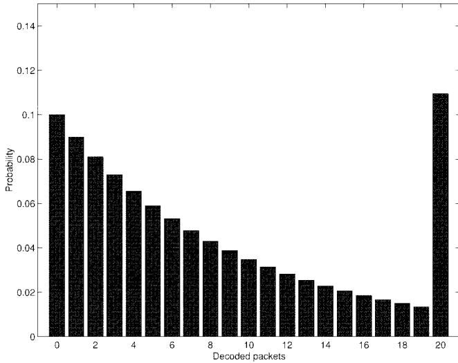
Fig. 1. Distribution of the number of decoded packets for 20 linearly dependent packets at 10% random loss.
