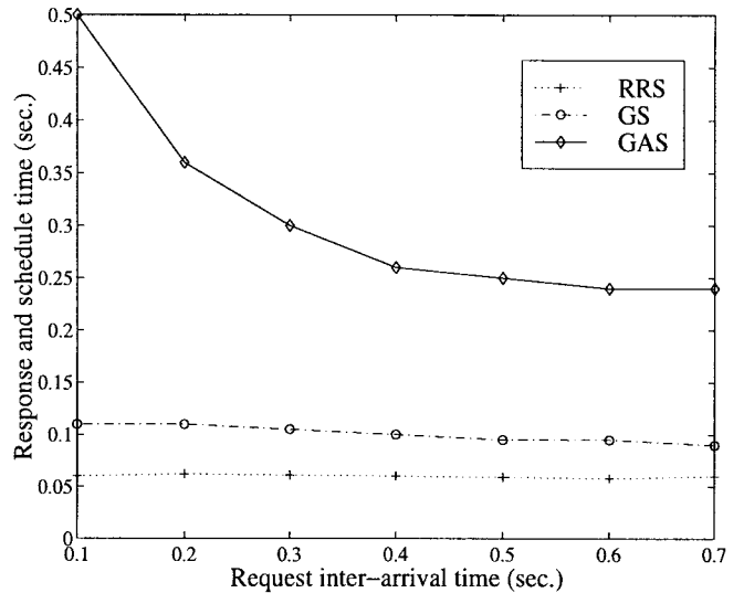
Fig. 20. Response and schedule time with user interactions.
