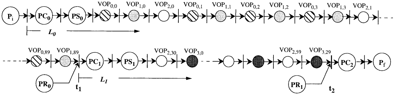
Fig. 6. MOCPN model for RRS scheduling.
