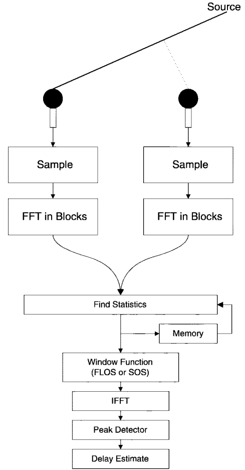
Fig. 7. Block diagram of the proposed TDE algorithm.
