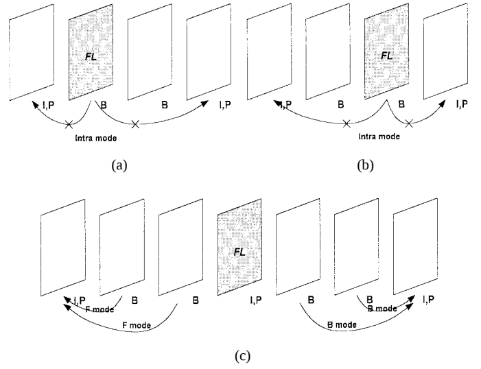
Fig. 6. Patterns of MB types in SGOP's with flashlights. (a) FLFB: flashlight lies at B_f . (b) FLRB: flashlight lies at B_r . (c) FLPI: flashlight lies at P or I.
