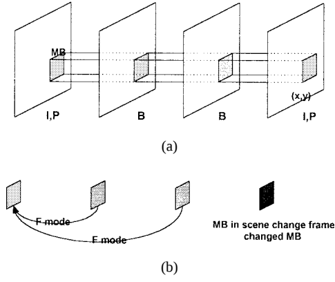
Fig. 3. (a) Illustration of MBGxy. (b) Example of pattern of MB type in the case of SCPI.
