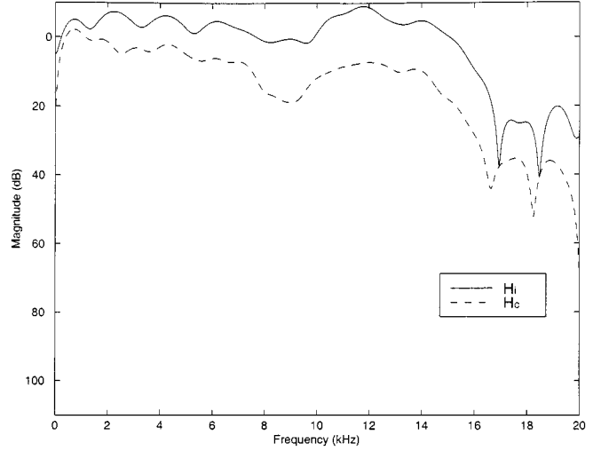
Fig. 10. The difference in dB between the ipsilateral ( H_i ) and the contralateral ( H_c ) terms shows the effect of head shadowing with no crosstalk cancellation. In this setup the loudspeakers were 50 cm apart and the head was located in the symmetric (center) position at a distance of 50 cm from the loudspeaker baffle plane.
