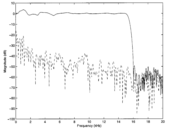
Fig. 11. Measured HRTF data from the loudspeakers ( H_i and H_c ) were used to simulate the physical system and design a set of filters to eliminate the crosstalk. The resulting diagonal (solid line) and off-diagonal (dotted line) terms produced by our simulation using the LMS method are plotted above. The diagonal term is very close to 1 (0 dB) from 2 to 15 kHz and deviates only slightly in the region below 1 kHz. The off-diagonal term starts at -15 dB and remains below -30 dB from 1 to 15 kHz.
