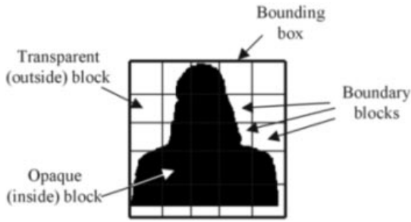
Fig. 1. Shape representation in MPEG-4.
