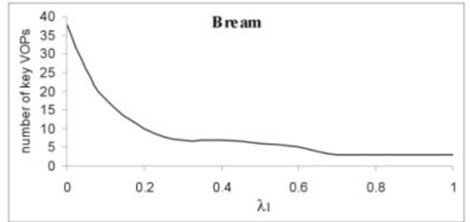
Fig. 5. Change in the number of key VOPs for different \lambda_1 values for the Breem video object.
