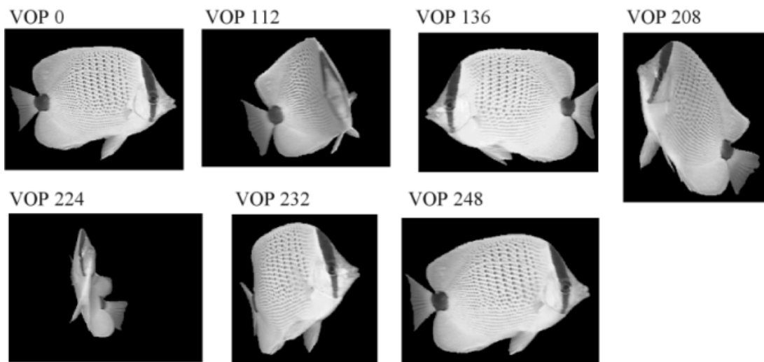
Fig. 10. Key VOPs selected using the Hausdorff distance based algorithm for the Bream video object.
