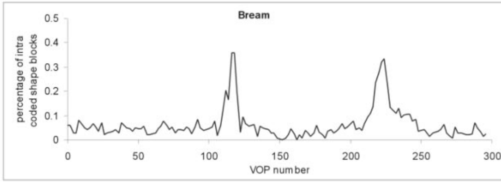
Fig. 6. Intra coded shape block activity for the Bream video object.
