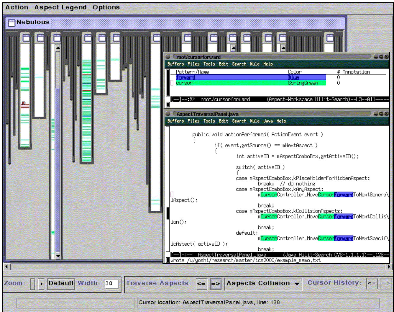
Figure 1. A screen shot of Aspect Browser being used on the Nebulous source. The top of the foreground panel is the aspect index, containing a pattern forward in blue and CURSOR in green, chosen to help find where code has to be added for a new traversal feature, based on conflict highlighting. Below the index is an Emacs buffer containing these aspects. In the background is Nebulous with aspect-less files folded under. The Nebulous cursor is about 2/3 down the first unfolded file from the left. The zooming and traversal features appear near the bottom, with the status bar below them.
