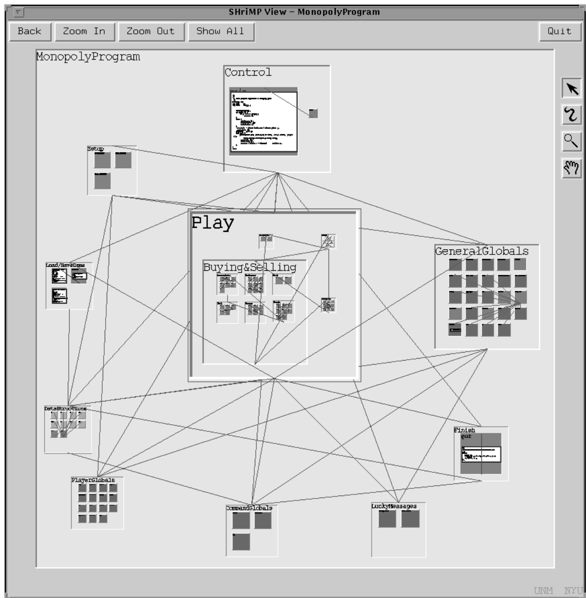
Figure 2: A SHriMP View.
